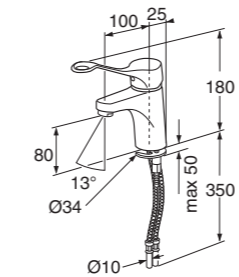
Nautic-pesuallashana, 160 mm vipu 214047-64 kromi
