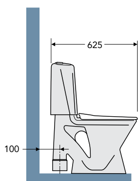
FLOOR-MOUNTED toilet
