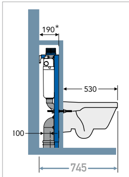
REPLACE WITH A WALL-MOUNTED TOILET ON A TRIOMONT FIXTURE
